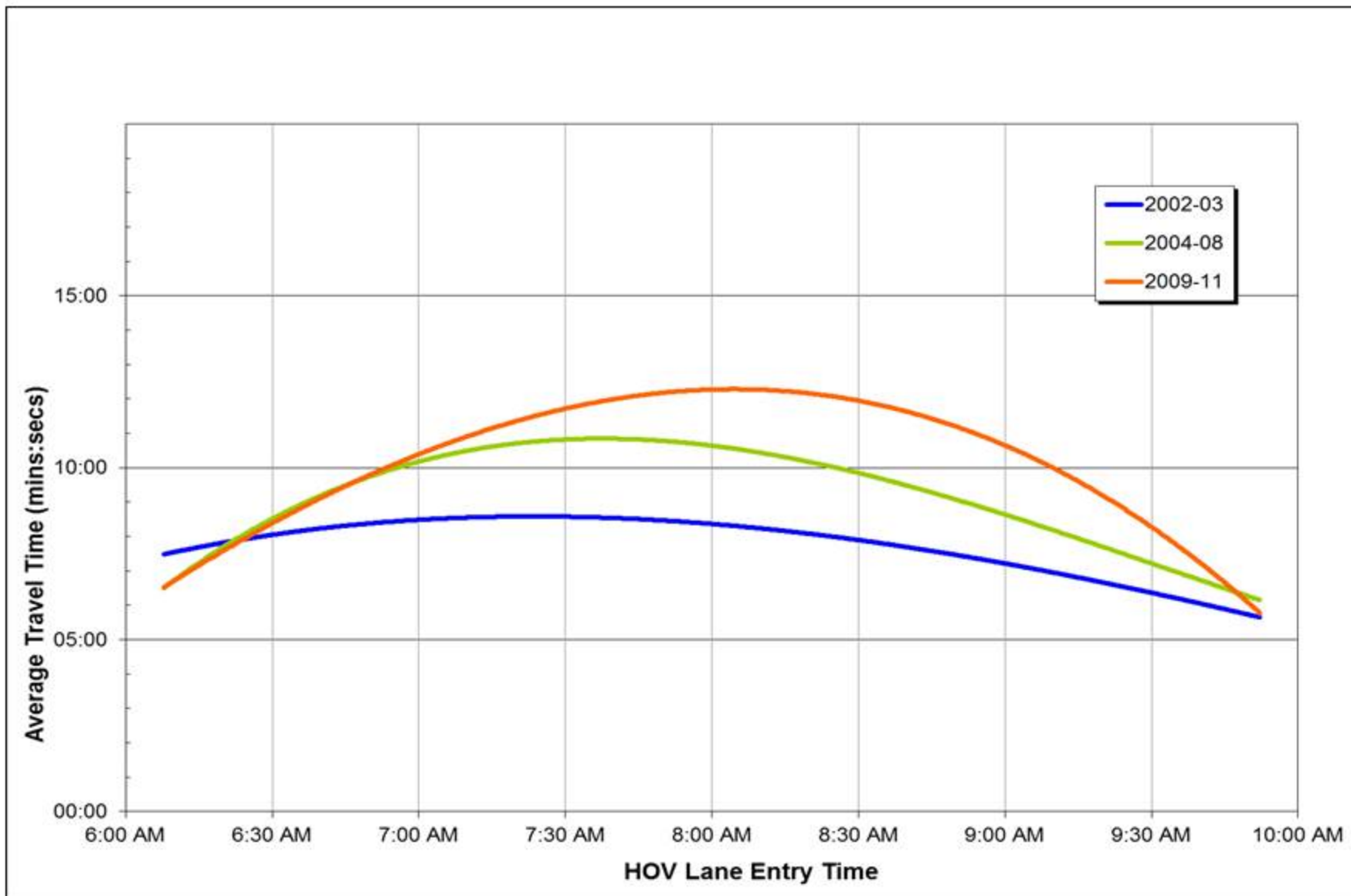
FIGURE 6 Southeast Expressway Travel Times: Northbound HOV Lane, AM Peak Period, 2002-11
