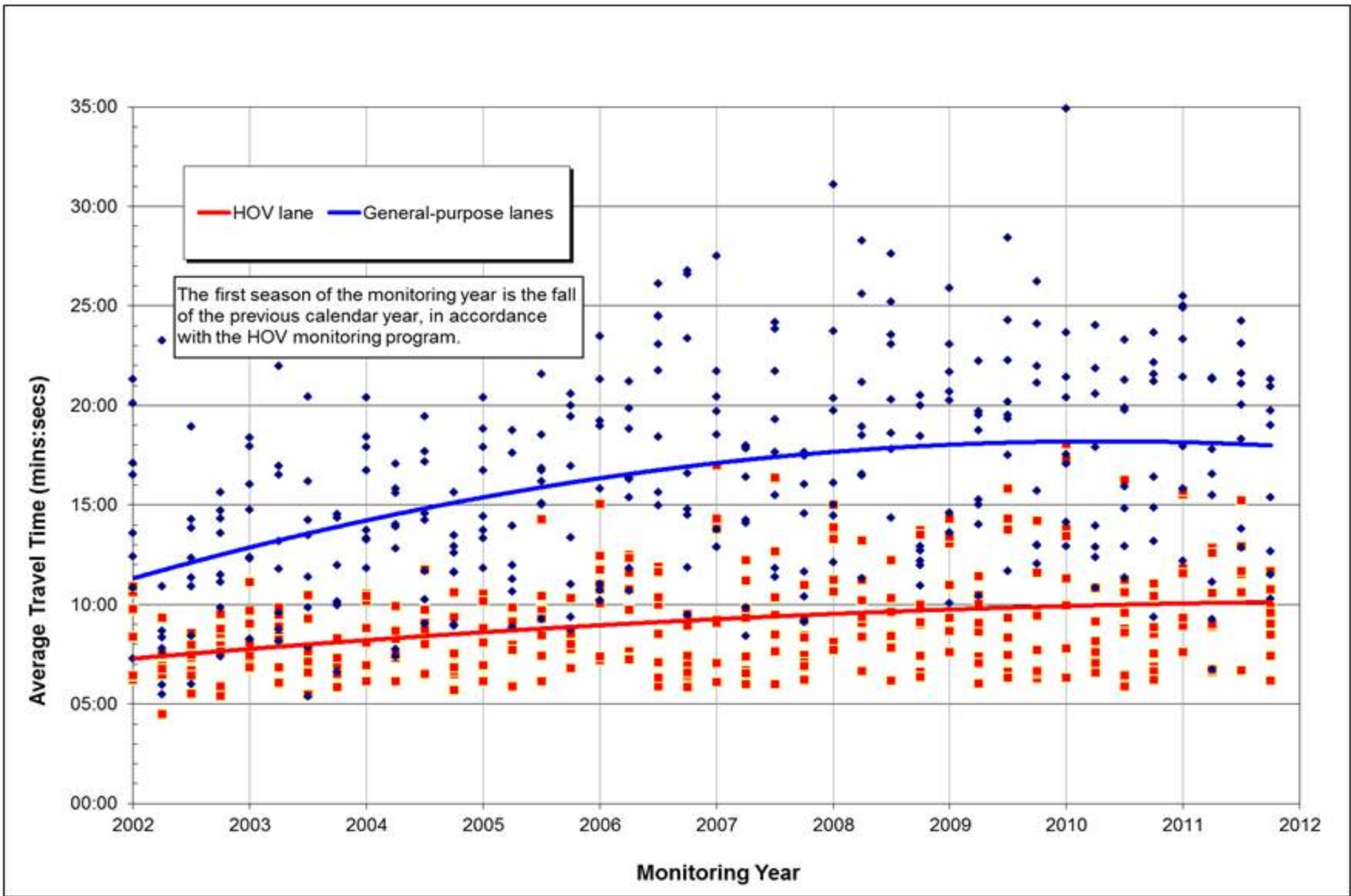
FIGURE 2 Southeast Expressway Travel Times: Northbound Travel Lanes, AM Peak Period, 2002-11
